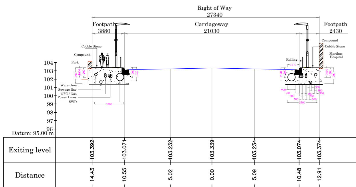
Cross Section at Chainage 400.00m
