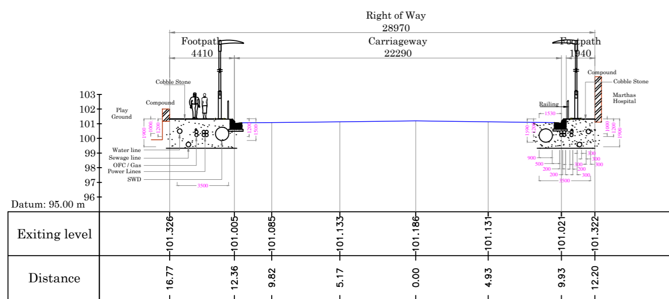
Cross Section at Chainage 250.00m
