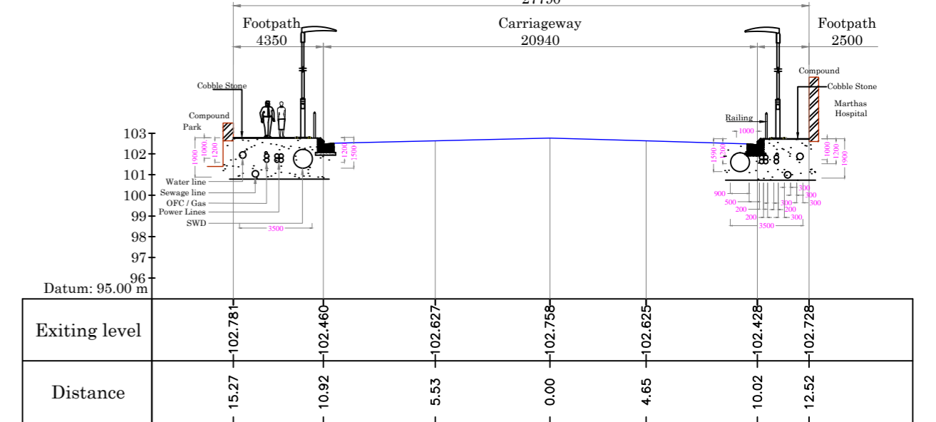
Cross Section at Chainage 350.00m
