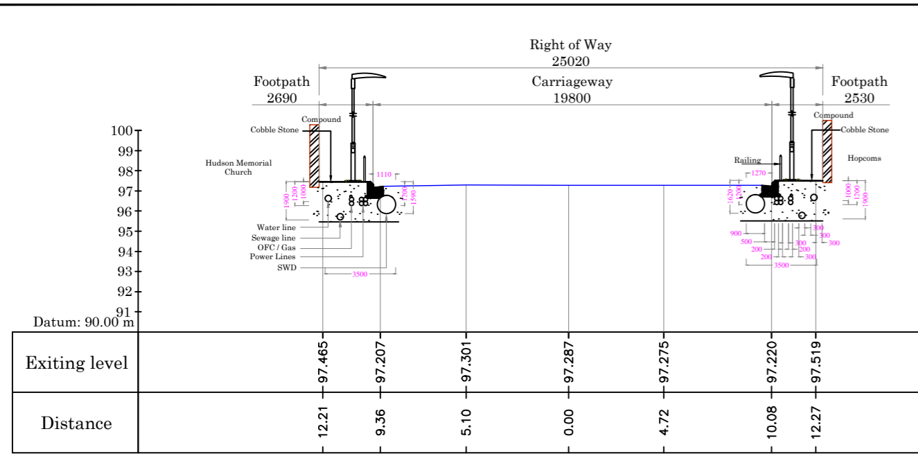
Cross Section at Chainage 50.00m
