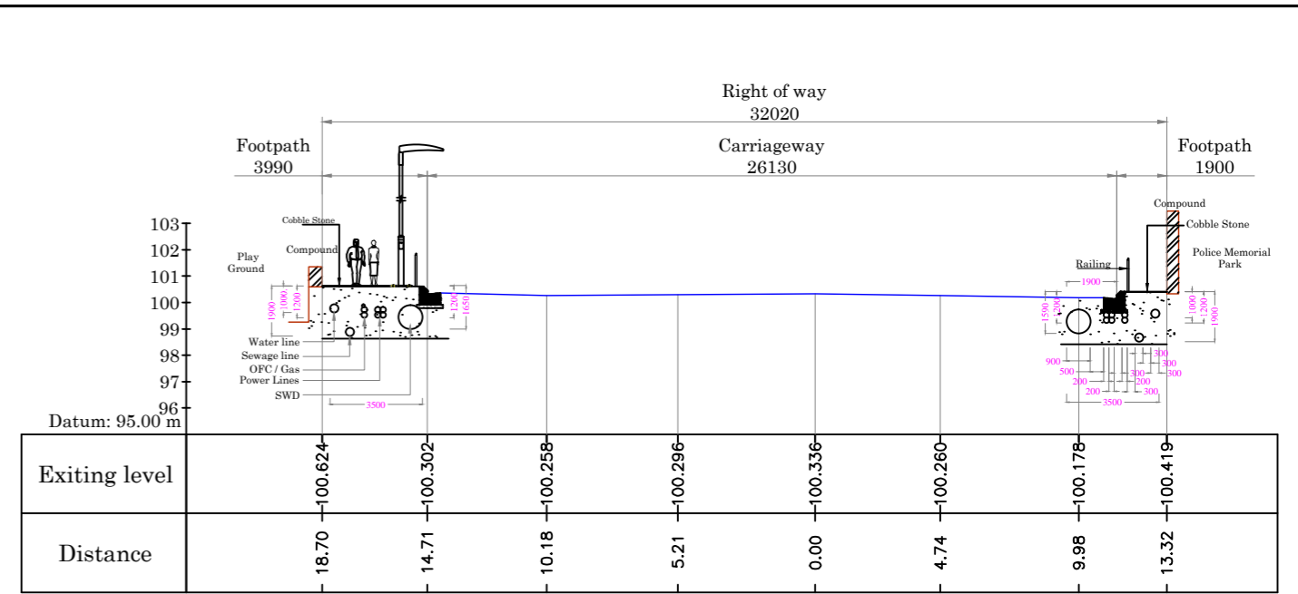
Cross Section at Chainage 200.00m
