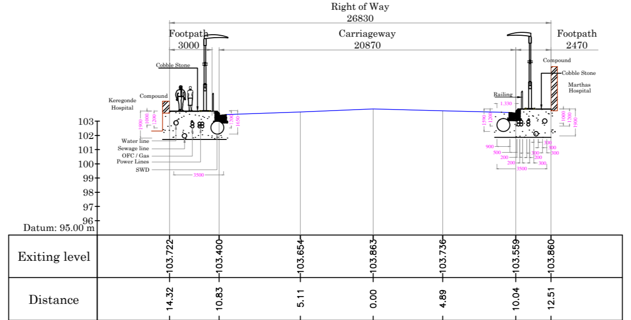
Cross Section at Chainage 450.00m
