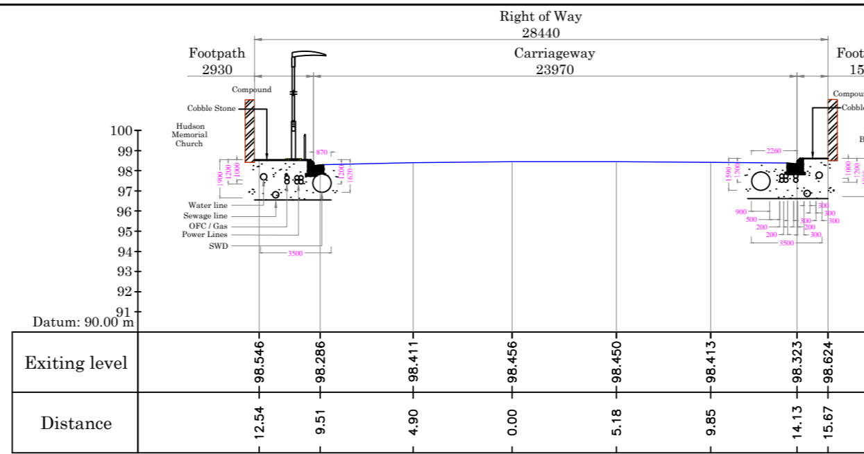
Cross Section at Chainage 100.00m
