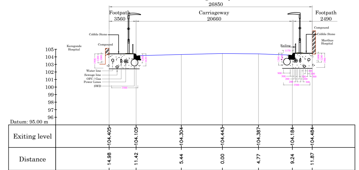
Cross Section at Chainage 500.00m
