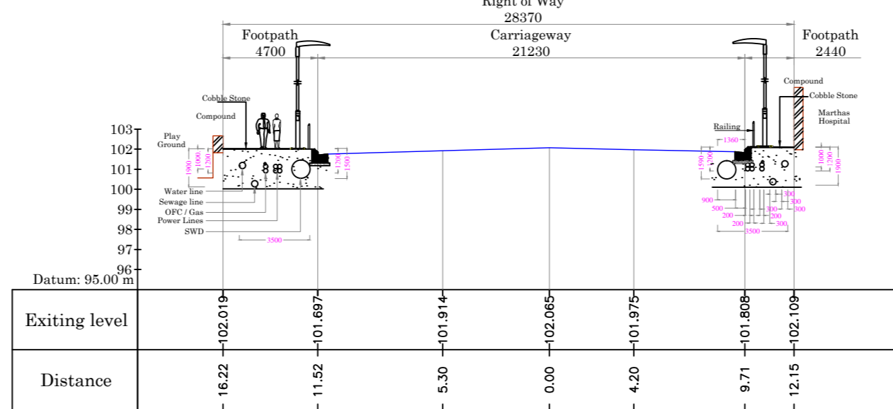
Cross Section at Chainage 300.00m
